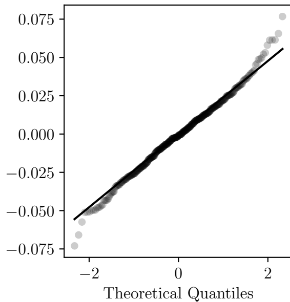
Mean Sample Quantiles
